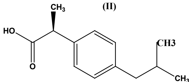
(S)-Ibuprofeno
